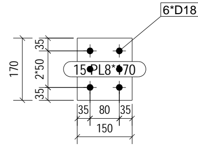
No. 8, Marked 15
