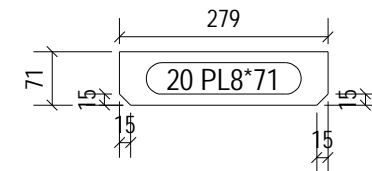
No. 24, Marked 20
