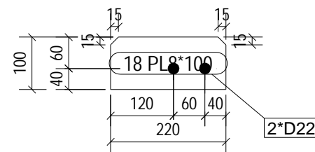
No. 24, Marked 18
