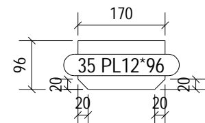
No. 24, Marked 35
