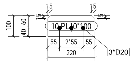
No. 16, Marked 10
