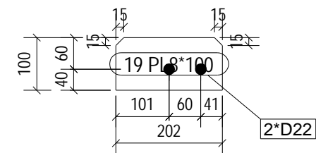
No. 8, Marked 19
