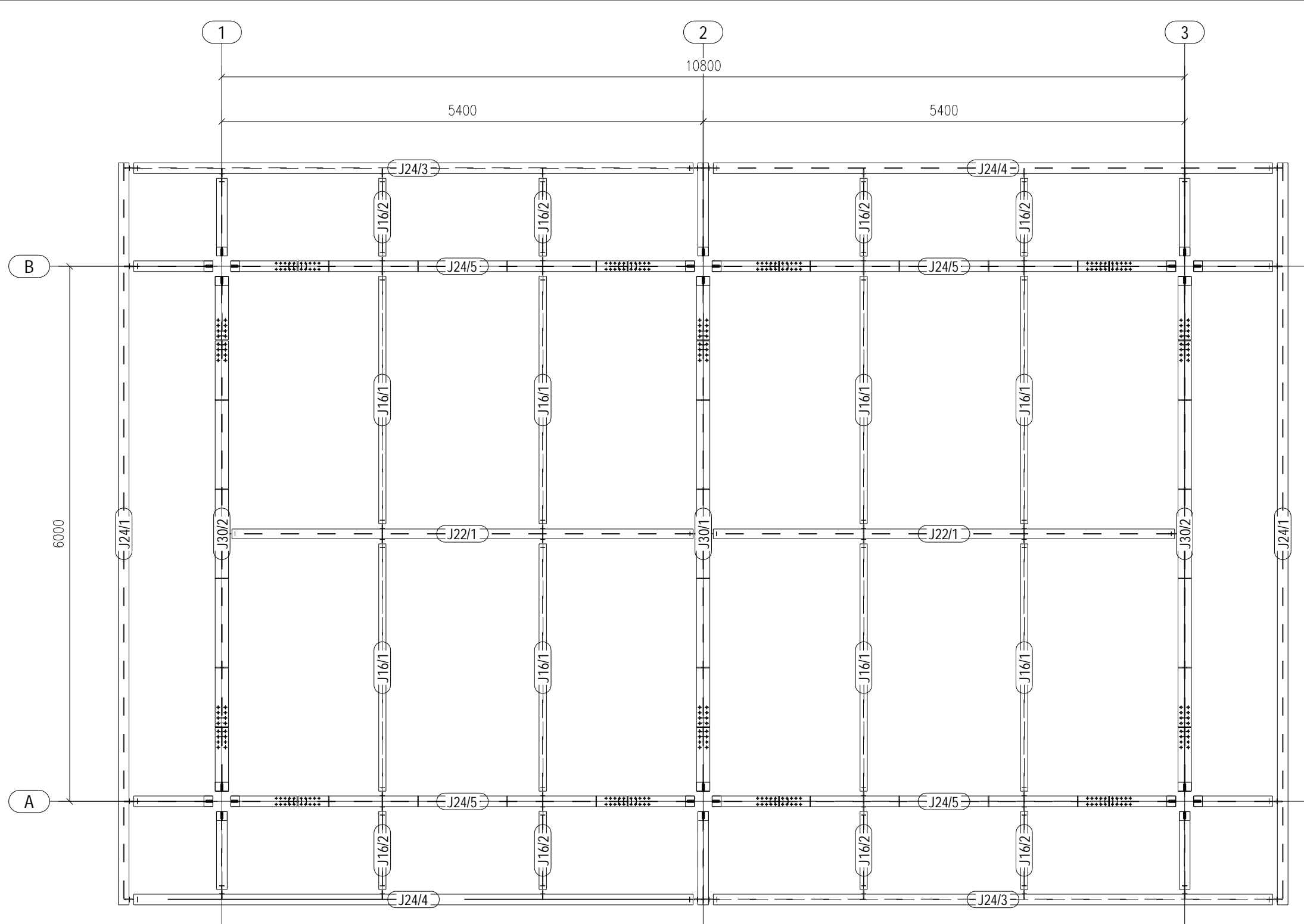
PLAN 3.17 1:50
