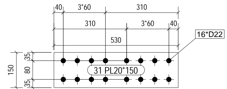
No. 12, Marked 31
