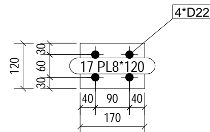
No. 64, Marked 17
